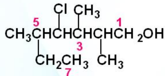
4-Chloro-2,3,5-trimethylheptan-1-ol
