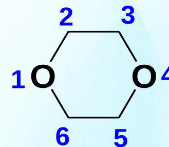
1,4-dioxane
